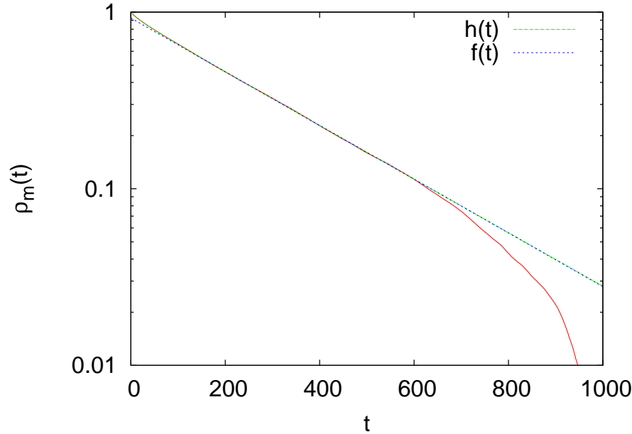
Figure 13.22: Fit of the autocorrelation function \rho_m(t) to the functions f(t) = c e^{-t/\tau} and h(t) = a_1 e^{-t/\tau_1} + a_2 e^{-t/\tau_2} + a_3 e^{-t/\tau_3} . For large times f(t) \approx h(t) , but h(t) is necessary in order to capture the small t behavior. This choice results in \tau_m = \tau = \tau_1 . The values of the parameters are given in the text. The vertical axes are in logarithmic scale.
