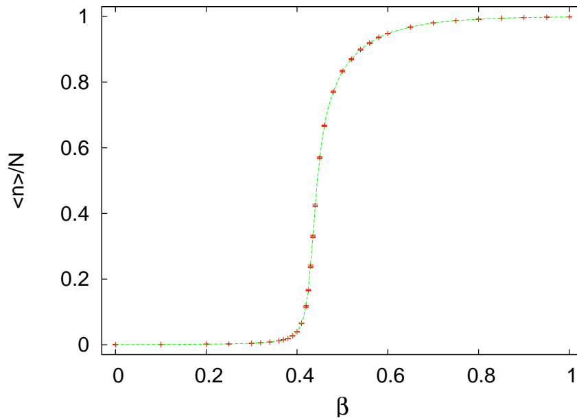
Figure 14.2: The Wolf cluster size as a function of the temperature. The plot shows the average cluster size as a fraction of the lattice size N . In the high temperature regime, \beta \ll \beta_c , this is \sim 1/N , and in the low temperature regime, \beta \gg \beta_c , it becomes \sim 1 . The data is for the Ising model on the square lattice for L = 40 .
