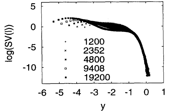
Figure 2. The SV(l) distributions for the c = 4 , \tau = 3 system. y = l/N^{1/\delta_h}
