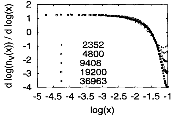
Figure 4. Short distance scaling of n_N(r) for c = 4 , \tau = 3 .
