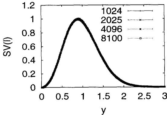
Figure 1. The SV(l) distributions for the c = 1/2 , \tau = 1 system. y = l/N^{1/\delta_h}
