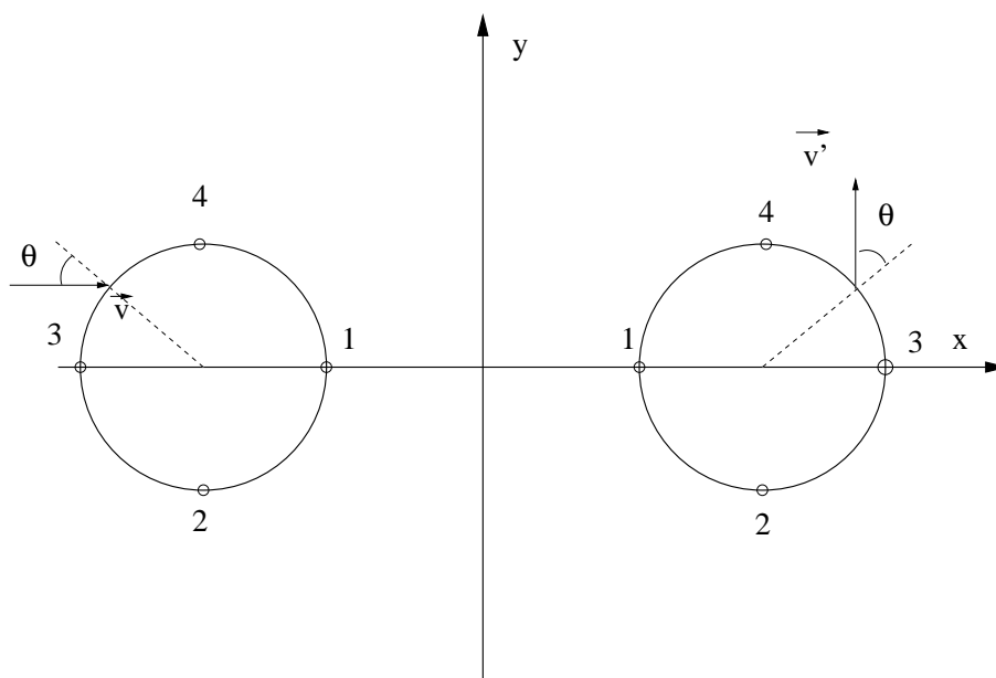
Figure 2.28: A simple model of the spacetime geometry of figure 2.27. The particle moves on the whole plane except withing the two disks that have been removed. The neck of the wormhole is modeled by the two circles x(\theta) = \pm d/2 \pm R \cos \theta , y(\theta) = R \sin \theta , -\pi < \theta \leq \pi and has zero length since their points have been identified. There is a given direction in this identification, so that points with the same \theta are the same (you can imagine how this happens by folding the plane across the y axis and then glue the two circles together). The entrance of the particle through one mouth and exit through the other is done as shown for the velocity vector \vec{v} \rightarrow \vec{v}' .
