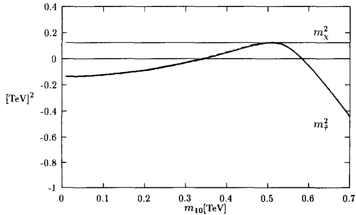
Fig. 6. The same as Fig. 4 for M = 0.8 TeV.
