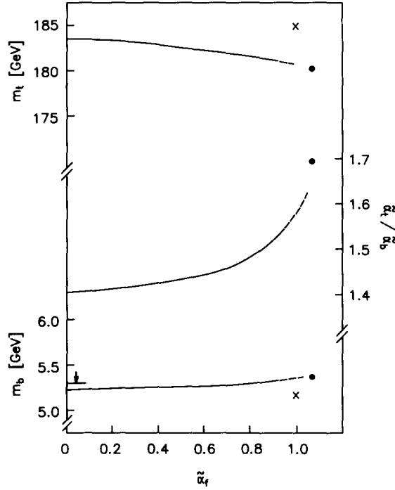
Fig. 1. The \tilde{\alpha}_f -dependence of \tilde{\alpha}_t and \tilde{\alpha}_b with \tilde{\alpha}_\lambda = 0 (Eqs. (41)). The values for the FUT |10| (Eqs.(44)) are indicated by \times . The \bullet points corresponds to \eta 's of the solution 3 (Eq. (40)).
