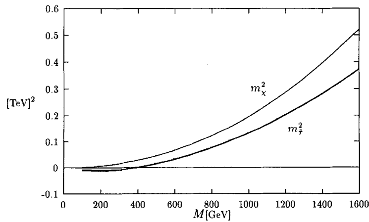
Fig. 4. m_7^2 and m_X^2 for the universal choice of the soft scalar masses.
