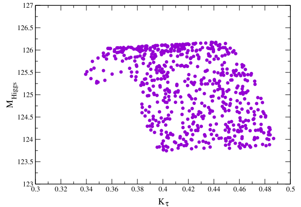
Fig. 4. The Higgs mass as a function of K_\tau = Y_\tau^2/g_3^2 .
