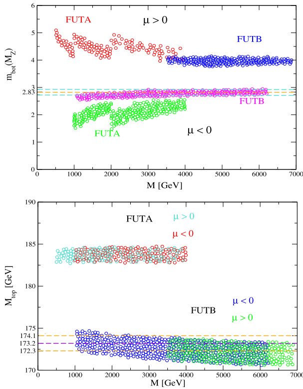
Fig. 1. The bottom quark mass at the Z boson scale (upper) and top quark pole mass (lower plot) are shown as function of M , the unified gaugino mass, for both models.
