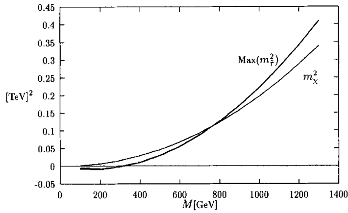
Fig. 8. \text{Max}(m_{\tau}^2) and m_{\chi}^2 as function of M .
