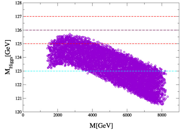
Fig. 2. The lightest Higgs mass, M_h , as function of M for the model FUTB with \mu < 0 , see text. (For interpretation of the references to colour, the reader is referred to the web version of this Letter.)
