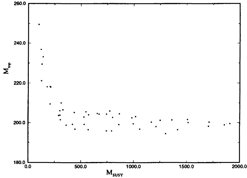
Fig. 2. The values for M_t predicted by the Pati-Salam model for different M_{\text{SUSY}} scales. Only the ones with M_{\text{SUSY}} beyond 400 GeV are realistic.
