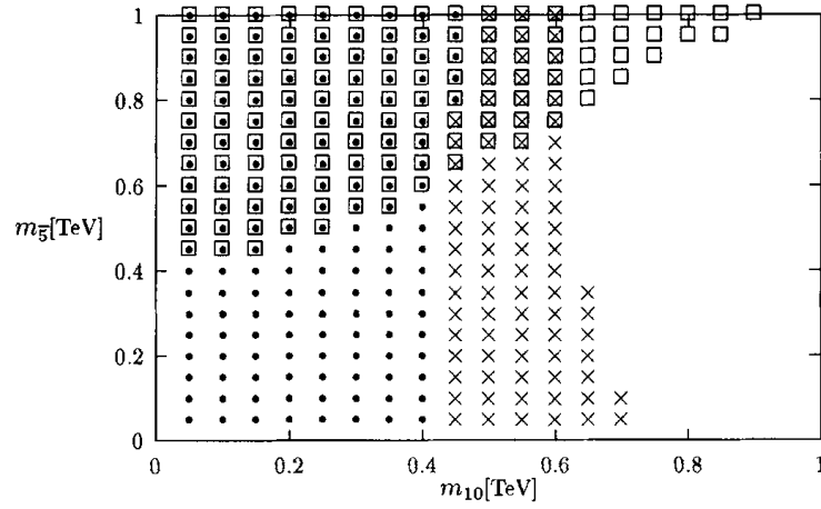
Fig. 3. The same as Fig. 1 with M = 1 TeV.
