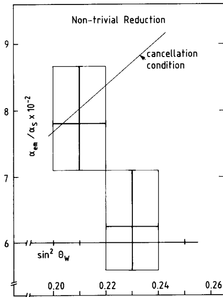
Fig. 1. Previous and recent experimental values and uncertainties of \sin^2\theta_w , \alpha_{em}/\alpha_s , compared with the cancellation condition.
