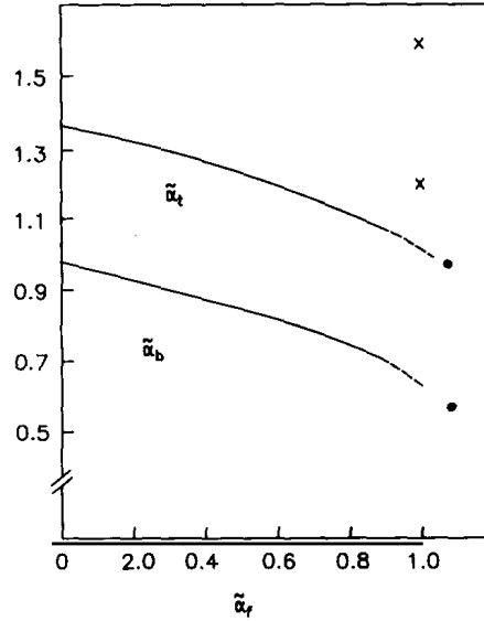
Fig. 2. The predictions of m_t , m_b and \tilde{\alpha}_t/\tilde{\alpha}_b ( m_{\text{GUT}} ) as functions of \tilde{\alpha}_f . The inputs are: m_{\text{SUSY}} = 200 GeV, \alpha_S(M_Z) = 0.12 , \alpha^{-1}(m_{\text{GUT}}) = 24.2 and m_\tau = 1.78 GeV. The points with \times are FUT predictions [10], and those with \bullet correspond to the edge of the solution 3 (Eq. (39)). The experimental upper bound on m_b is also indicated.
