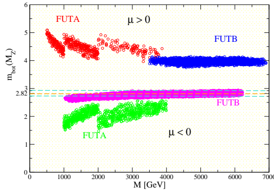
Figure 1: \bar{m}_b(M_Z) as function of M for models FUTA and FUTB , for \mu < 0 and \mu > 0 .
