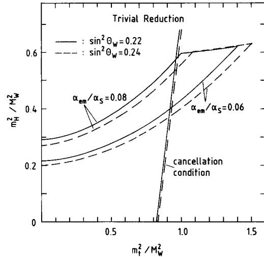
Fig. 2. Range of m_H^2/M_w^2 versus m_t^2/M_w^2 for the trivial reduction.
