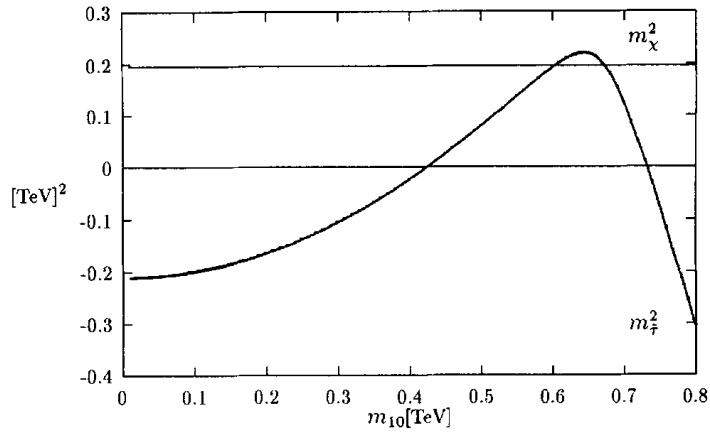
Fig. 7. The same as Fig. 4 for M = 1 TeV.
