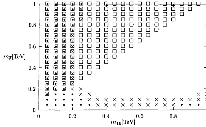
Fig. 1. The region without squares, dots and crosses yields a neutralino as the LSP for model A with M = 0.3 TeV.
