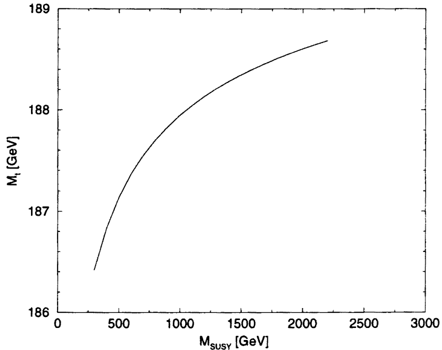
Fig. 3. M_t prediction versus M_{\text{SUSY}} for \tilde{\alpha}_T = 2.717 .
