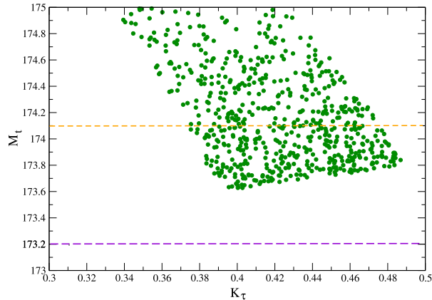
Fig. 2. The top mass as a function of K_\tau = Y_\tau^2/g_3^2 , the purple dashed line is the experimental central value and the orange one is the 1\sigma value. (For interpretation of the references to colour in this figure legend, the reader is referred to the web version of this article.)
