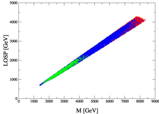
Fig. 3. The mass of the LOSP is presented as a function of M . Shown are only points that fulfill the B -physics constraints. The green (light shaded) points correspond to M_h = 126 \pm 1 GeV, the blue (dark shaded) points have M_h = 126 \pm 3 GeV, and the red points have no M_h restriction. (For interpretation of the references to colour, the reader is referred to the web version of this Letter.)
