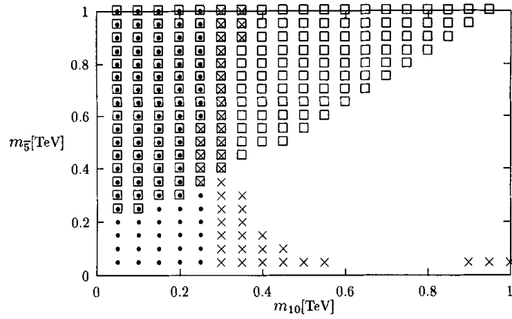
Fig. 2. The same as Fig. 1 with M = 0.5 TeV.
