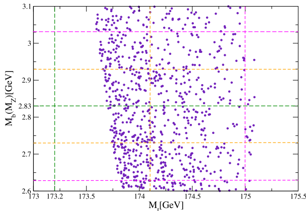
Fig. 3. Using the regions of values for K_\tau = Y_\tau^2/g_3^2 and \tan\beta which give experimentally accepted tau mass, this figure shows the resulted points in the (M_t, M_b) phase space. The central value (green dashed lines), as well as the 1 and 2\sigma deviation (orange and magenta lines respectively), for the top and bottom masses is also drawn. (For interpretation of the references to colour in this figure legend, the reader is referred to the web version of this article.)
