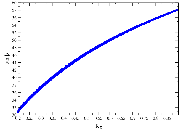
Fig. 1. Required values of \tan \beta as a function of K_\tau = Y_\tau^2/g_3^2 in order to get the experimentally accepted tau mass.
