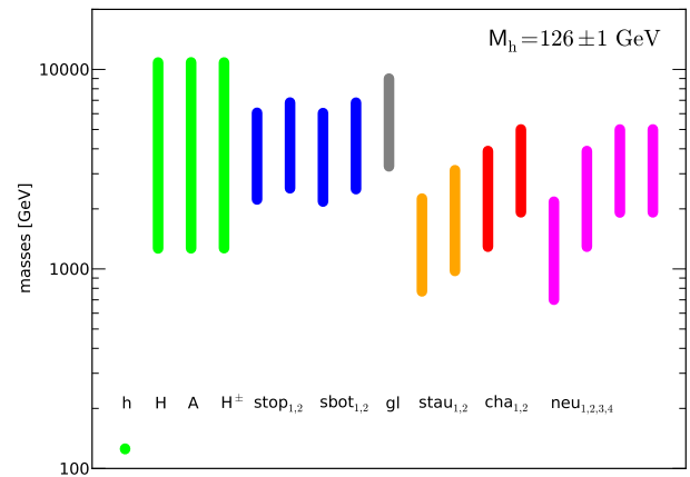
Fig. 4. The upper (lower) plot shows the spectrum after imposing the constraint M_h = 126 \pm 3(1) GeV. The particle spectrum of model FUTB with \mu < 0 , where the points shown are in agreement with the quark mass constraints and the B -physics observables. The light (green) points on the left are the various Higgs boson masses. The dark (blue) points following are the two scalar top and bottom masses, followed by the lighter (grey) gluino mass. Next come the lighter (beige) scalar tau masses. The darker (red) points to the right are the two chargino masses followed by the lighter shaded (pink) points indicating the neutralino masses. (For interpretation of the references to colour in this figure legend, the reader is referred to the web version of this Letter.)
