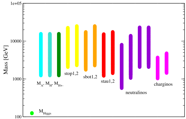
Fig. 5. The Higgs mass and s-spectrum for values of M_U \sim 1.3 TeV to \sim 11 TeV.
