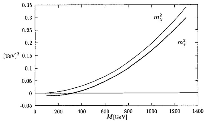
Fig. 9. m_{\tau}^2 and m_{\chi}^2 as function of M for the universal choice.
